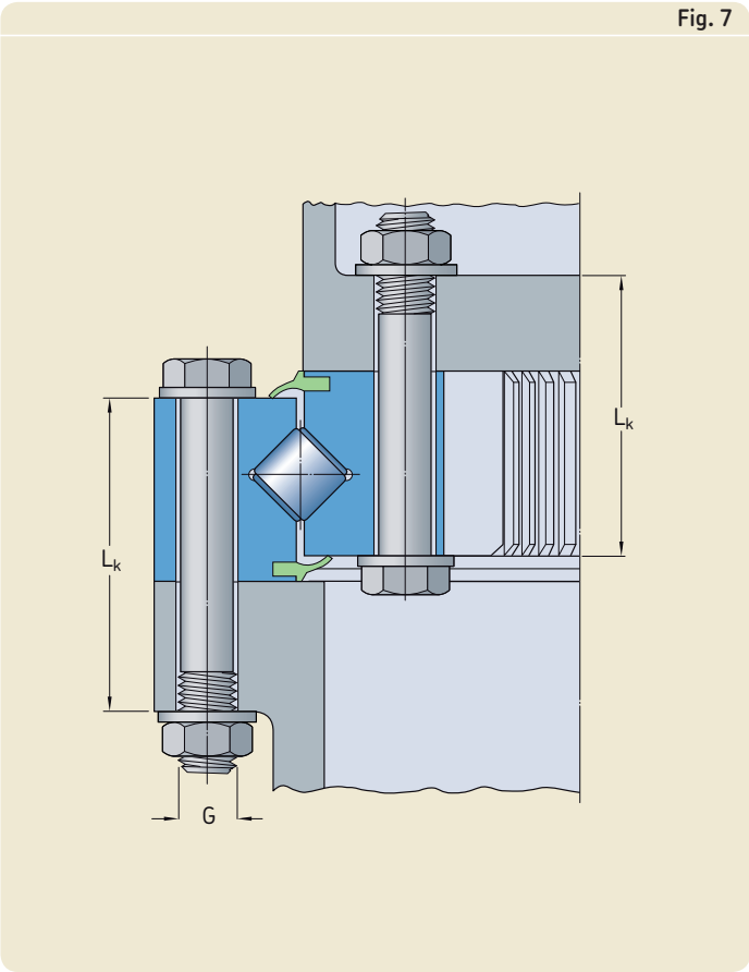
Fig. 7 Bolt joints
