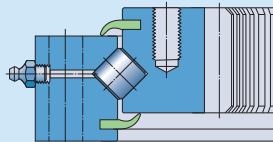
162 series with an internal gear
