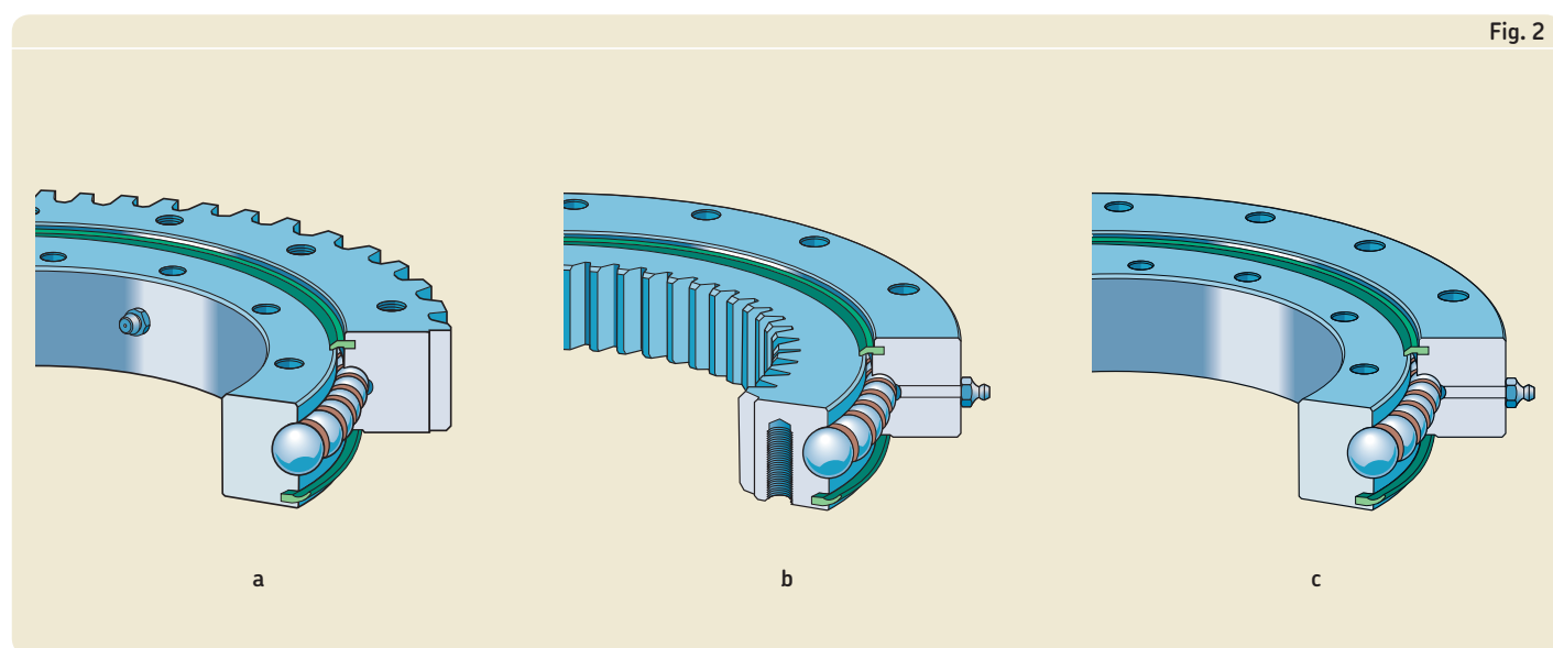
Medium size four-point contact ball slewing bearings
