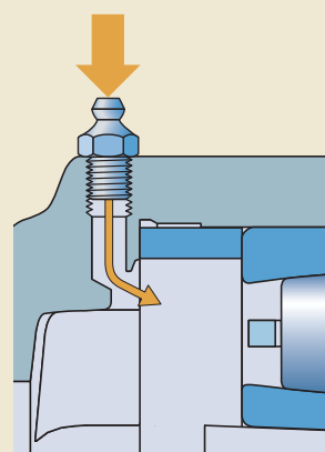
Grease guiding system
