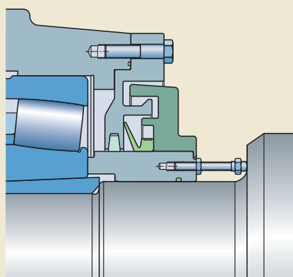
Labyrinth seal with one V-ring seal
