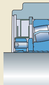
Labyrinth seal (for SKF ConCentra)
