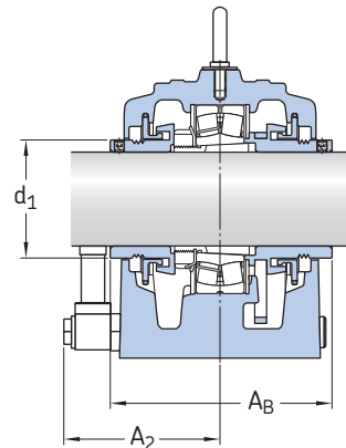
Housing for through shaft
