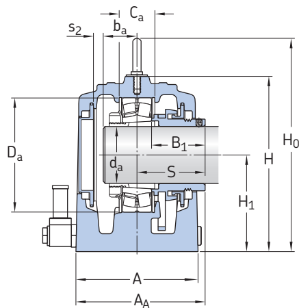
Housing for shaft end
