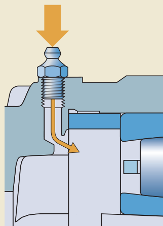
Relubrication from the side
