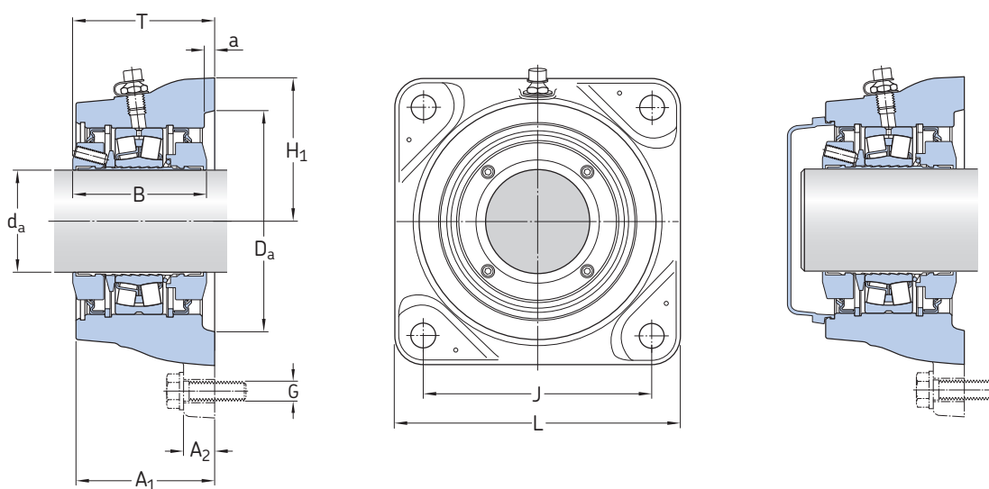
Housing design for shaft diameters 65 to 100 mm
