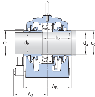
Housing for through shaft
