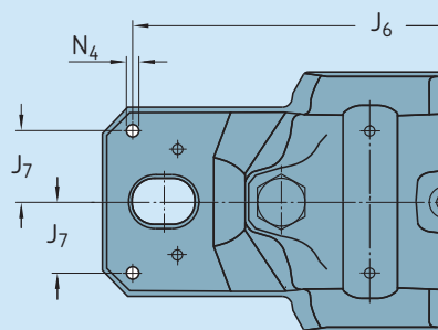
Position and size of dowel pin holes
