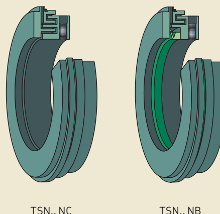
Taconite heavy-duty seals
