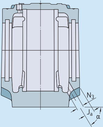
Recommended dimensions for grease escape holes
