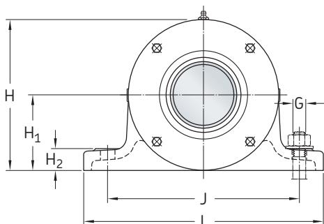
Sizes up to and including 211 and 309
