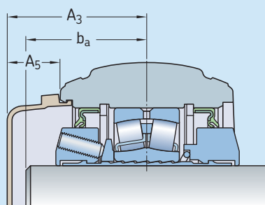
SYNT series
