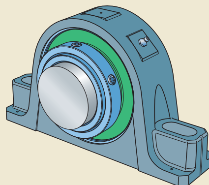
SYR series
