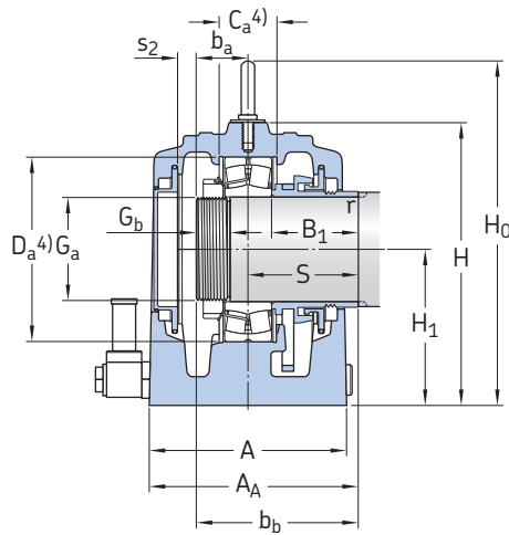
Housing for shaft end
