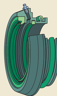
Taconite seal TER...
