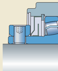
Labyrinth seal (for collar-mount)
