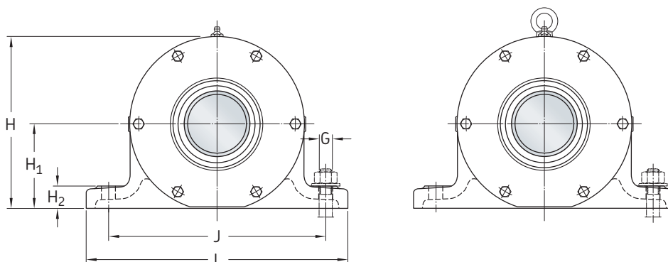
Size 320 and above (with M10 eye bolt)
