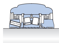
High-speed variant Designation suffix TS
