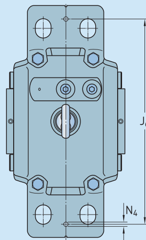
Position and size of dowel pin holes
