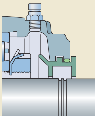
Seal for large axial movements
