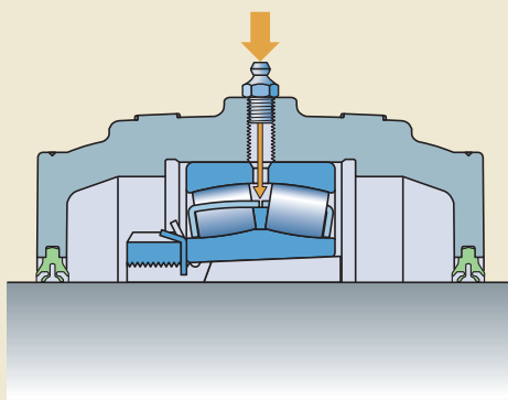
Relubrication via the outer ring
