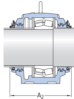
Taconite seals, TNF design
