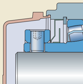
End plug
