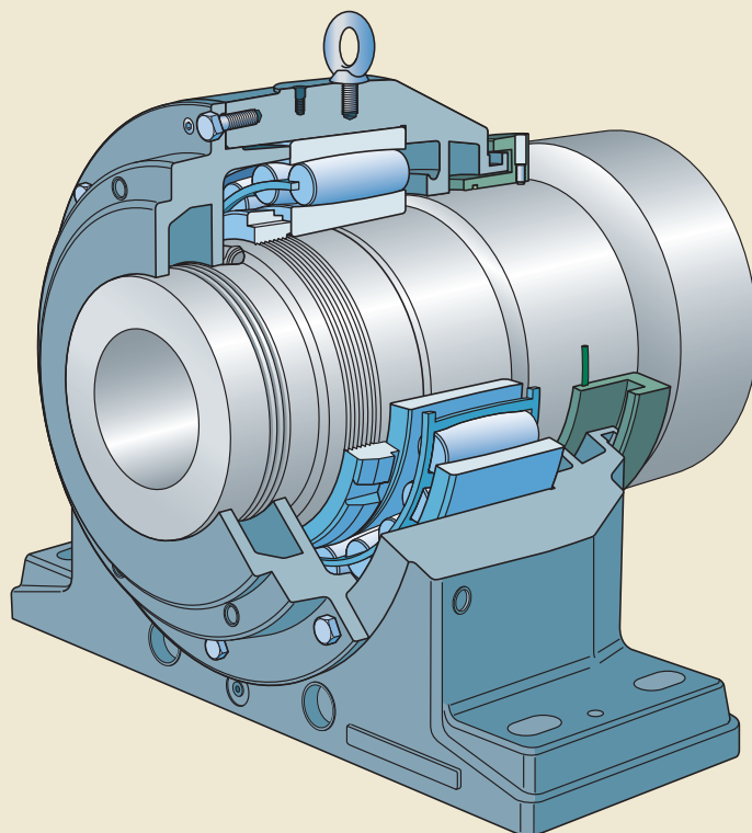
Housing for steam joint connection, SBPN series
