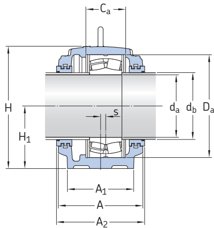
Labyrinth seals, TS design
