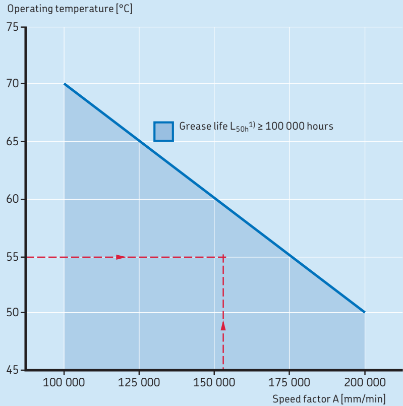
Temperature-speed relationship for relubrication-free SKF ConCentra roller bearing units
