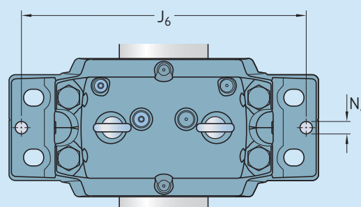
Position and size of dowel pin holes
