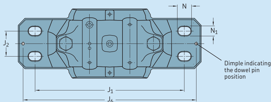
Dimensions for four cast attachment bolt holes
