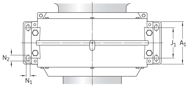
SDM..RA
