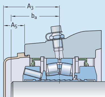
FYNT series
