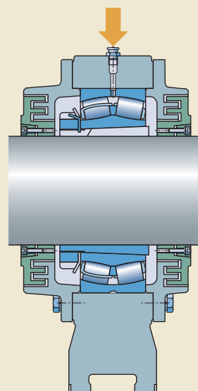
Grease fitting in THD housing
