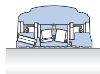
Relubrication-free variant Designation suffix W
