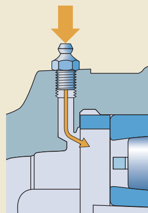
Relubrication from the side
