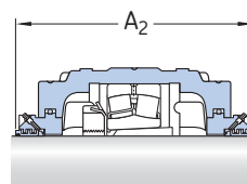
with TSN .. ND
