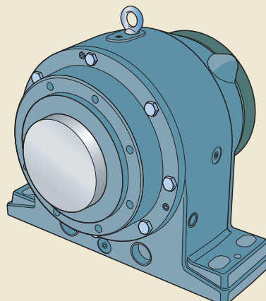
SBPN drying cylinder housings
