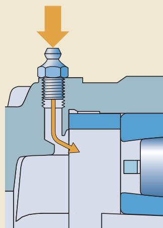
Grease guiding system
