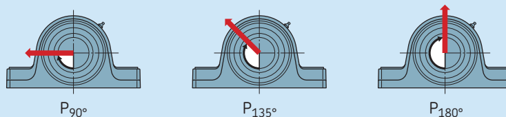
Safe loads for FSYE series roller bearing units
