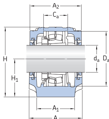
with TSN .. A
