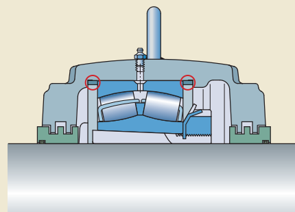
Locating bearing held axially by locating rings
