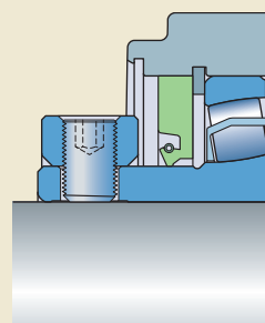
Radial shaft seal
