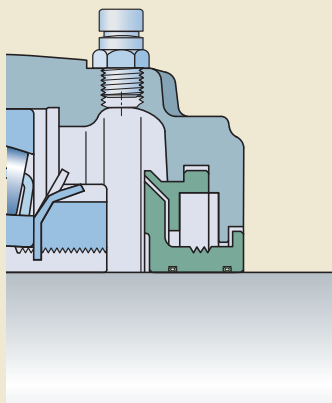
Housing for oil lubrication
