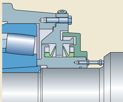
Labyrinth seal with two V-ring seals
