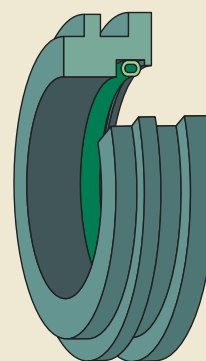
Labyrinth ring TSN .. S
