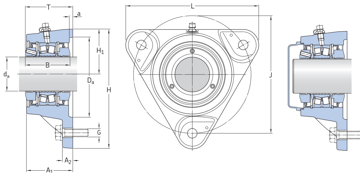
Housing design for shaft diameters 35 to 60 mm
